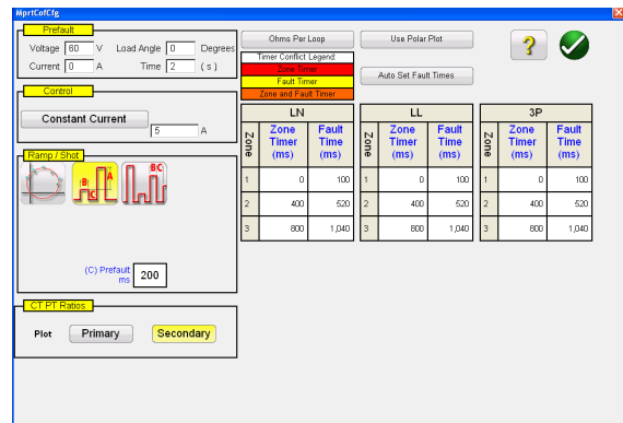
Generic QUAD Test Setup Screen
