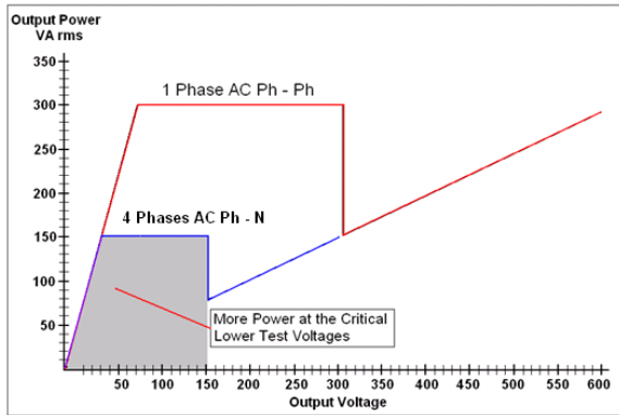
Voltage Output Power Curve
